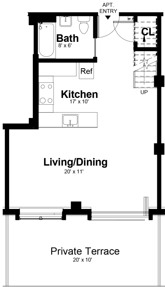
UNIT F - FIRST FLOOR
