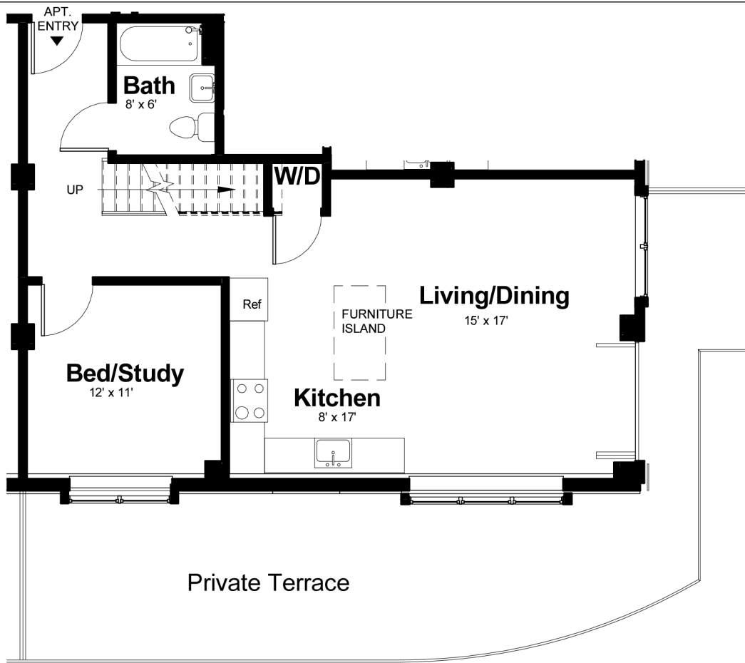
UNIT G - FIRST FLOOR
